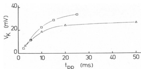
FIGURE 2 V_K shifts in frog node and squid giant axon during comparable depolarizing pulses, V_{pp} , as a function of prepulse duration, t_{pp} : (Δ) myelinated fiber of frog (fiber 5373, V_{pp} = 70 mV); (□) giant axon of squid (from Fig. 2 a of Palti et al., 1972; E_H = -59 mV, V_{pp} = 65 mV).
